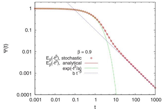
FIG. 2. (Color online) The Mittag-Leffler complementary cumulative distribution function sampled from Eq. (20) (circles) and computed analytically (solid line) [39], as well as its approximations for t \rightarrow 0 (Weibull function, long dashes) and t \rightarrow \infty (power law, short dashes).
