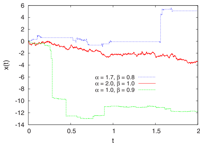
FIG. 1. (Color online) Sample paths of CTRWs with scale parameters \gamma_t=0.001 , \gamma_x=\gamma_t^{\beta/\alpha} , and different choices of \alpha and \beta . With smaller \alpha the jumps become larger; with smaller \beta the waiting times become longer.
