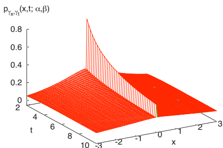
FIG. 3. (Color online) Decay of the probability density P_{\gamma_x, \gamma_t}(x, t; \alpha, \beta) with \alpha=1.7, \beta=0.8, \gamma_t=0.1 , and \gamma_x = \gamma_t^{\beta/\alpha} . The crest at x=0 is the survival function \Psi(t) = E_\beta(-t/\gamma_t)^\beta = P(0^+, t) - P(0^-, t) , where P(x, t) = \int_{-\infty}^x p(u, t) du .
