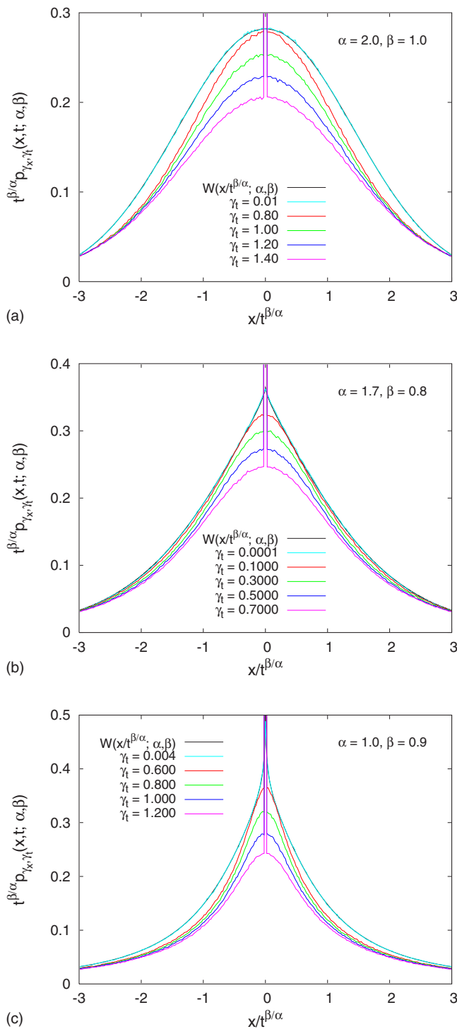
FIG. 4. (Color online) Convergence of t^{\beta/\alpha} p_{\gamma_x, \gamma_t}(x, t; \alpha, \beta) to the scaling function W(x/t^{\beta/\alpha}; \alpha, \beta) , Eq. (8), at t=2 for selected values of \alpha and \beta . The curves are shown in a time-independent way as scaling plots and appear in the same order from bottom to top as reported in the legend—i.e., with decreasing \gamma_t . The curve with the smallest \gamma_t is almost indistinguishable from its theoretical limit W (solid black line). However, in spite of the impression that may arise from the few terms and the ranges chosen here, in general the function sequences are not monotonic. The scale parameters \gamma_x and \gamma_t tend to 0 as \gamma_x^\alpha = \gamma_t^\beta . The central peak decreases when the ratio t/\gamma_t becomes larger, as is evident in Fig. 3.
